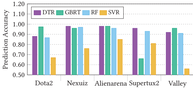
Figure 4: Prediction accuracy of machine learning model
