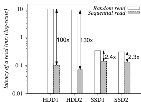
Figure 1: Read latency on two HDDs and two SSDs (for commercial reasons, we do not disclose the brands of the disks). Each read fetches 4KB. The OS buffer is by-passed.
