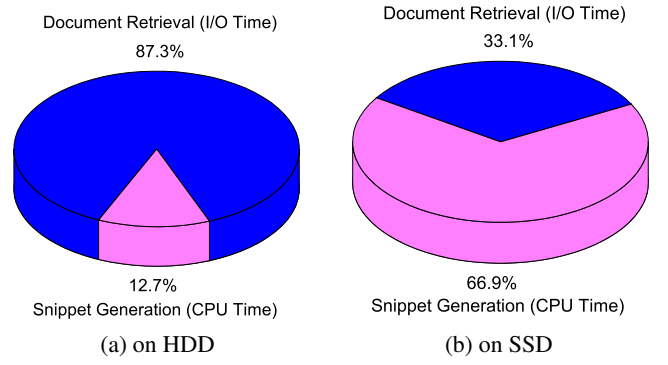
Figure 9: Document retrieval time vs. snippet generation in a document server
