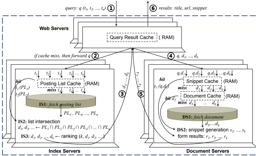
Figure 2: Web search engine architecture
